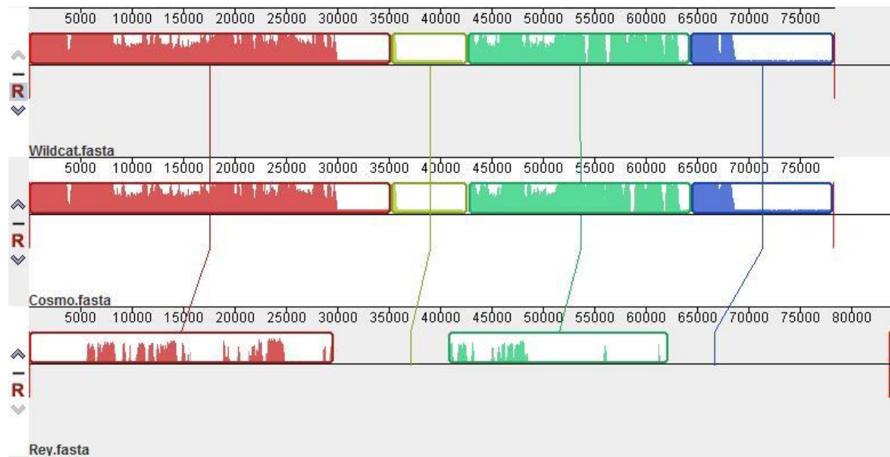
Fig. 3. progressiveMauve alignment (2) of the genomes of the members of the genus Wildcatvirus and their closest relative phage Mycobacterium phage Rey. Colored blocks indicate the regions of 1 to 1 best alignment with rearrangement breakpoints in a different random color. The degree of sequence similarity between regions is given by a similarity plot within the colored blocks with the height of the plot proportional to the average nucleotide identity (Aaron Darling, personal communication).
