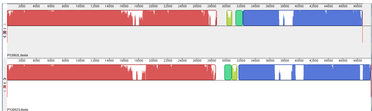
Fig. 2. progressiveMauve alignment [1] of the annotated genomes of members of the P12002virus genus – from top to bottom: Polaribacter phages P12002L and P12002S. Colored blocks indicate the regions of 1 to 1 best alignment with rearrangement breakpoints in a different random color. The degree of sequence similarity between regions is given by a similarity plot within the colored blocks with the height of the plot proportional to the average nucleotide identity (Aaron Darling, personal communication).
