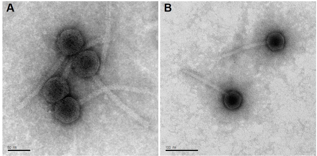
Fig. 1. Electron micrograph of negatively stained, uranyl acetate, Polaribacter phages P12002L (A) and P12002S (B) (provided by Jang-Cheon Cho).
