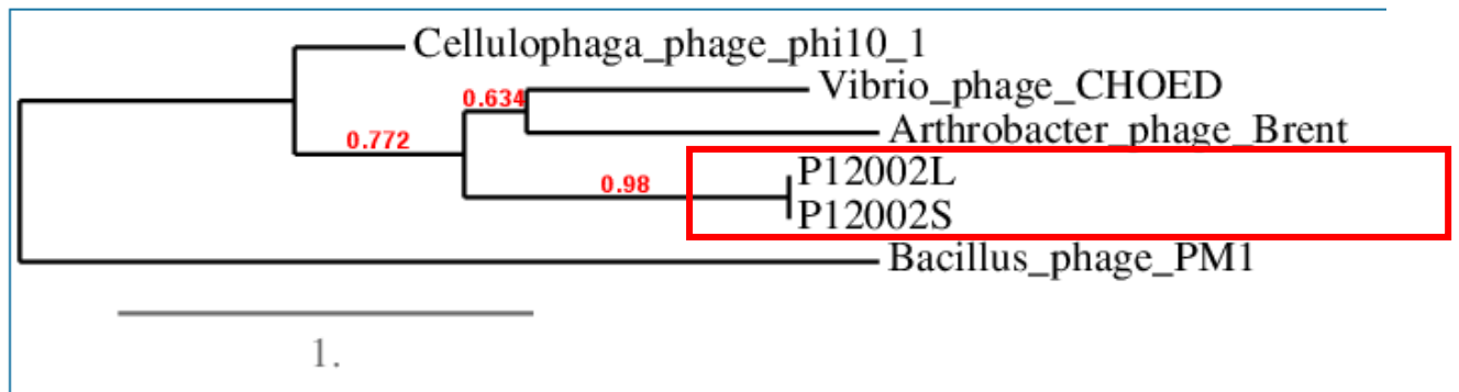
Figure 1: Phylogenetic tree (the branch length is proportional to the number of substitutions per site).
