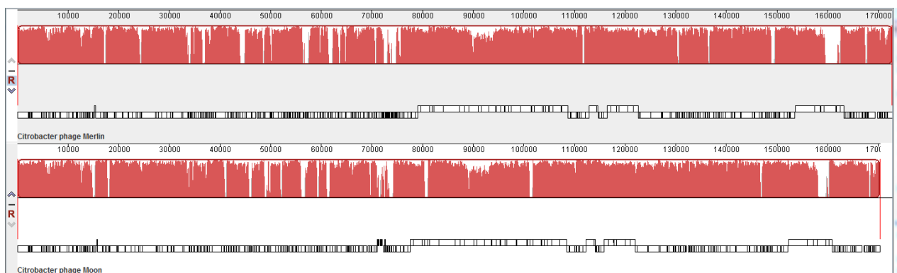
Fig. 2. progressiveMauve alignment [1] of the annotated genomes of members of the Moonvirus genus – from top to bottom: Citrobacter phages Merlin and Moon. Colored blocks indicate the regions of 1 to 1 best alignment with rearrangement breakpoints in a different random color. The degree of sequence similarity between regions is given by a similarity plot within the colored blocks with the height of the plot proportional to the average nucleotide identity (Aaron Darling, personal communication).
