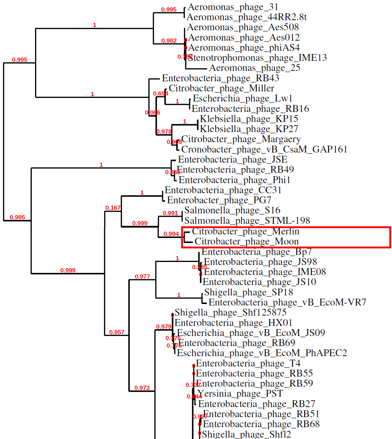
Fig. 3. Phylogenetic analysis of large subunit terminase proteins of viruses related to Citrobacter phage Moon constructed using “one click” at phylogeny.fr [3]. "The "One Click mode" targets users that do not wish to deal with program and parameter selection. By default, the pipeline is already set up to run and connect programs recognized for their accuracy and speed (MUSCLE for multiple alignment and PhyML for phylogeny) to reconstruct a robust phylogenetic tree from a set of sequences." It also includes the use of Gblocks to eliminate poorly aligned positions and divergent regions. "The usual bootstrapping procedure is replaced by a new confidence index that is much faster to compute. See: Anisimova M., Gascuel O. Approximate likelihood ratio test for branches: A fast, accurate and powerful alternative (Syst Biol. 2006;55(4):539-52.) for details."
