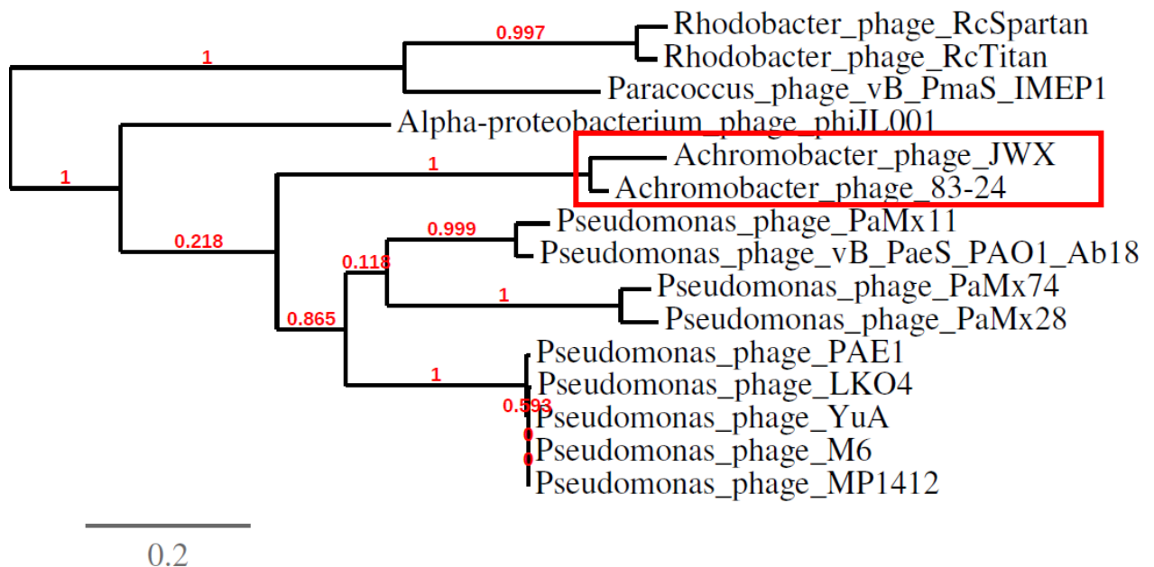
Fig. 3. Phylogenetic analysis of the large subunit terminase proteins of the members of the genus Jwxvirus and related viruses constructed using “one click” at phylogeny.fr [3]. "The "One Click mode" targets users that do not wish to deal with program and parameter selection. By default, the pipeline is already set up to run and connect programs recognized for their accuracy and speed (MUSCLE for multiple alignment and PhyML for phylogeny) to reconstruct a robust phylogenetic tree from a set of sequences." It also includes the use of Gblocks to eliminate poorly aligned positions and divergent regions. "The usual bootstrapping procedure is replaced by a new confidence index that is much faster to compute. See: Anisimova M., Gascuel O. Approximate likelihood ratio test for branches: A fast, accurate and powerful alternative (Syst Biol. 2006;55(4):539-52.) for details."
